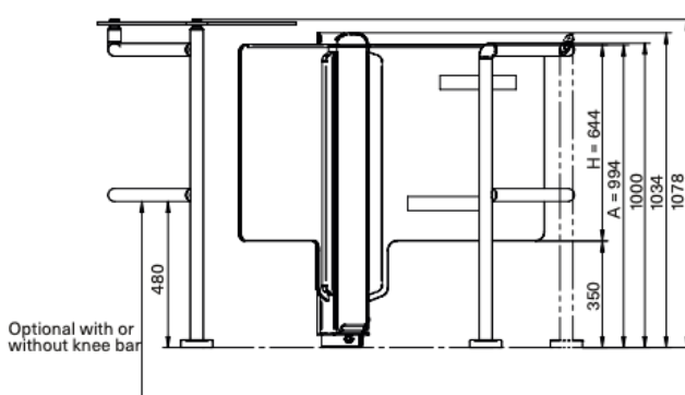
mTwing with glass panels – side view
