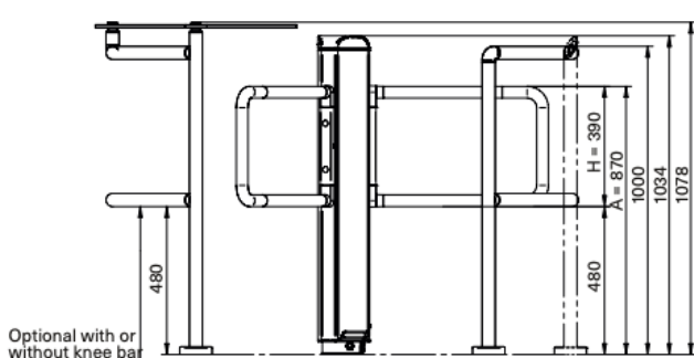
mTwing with U-bars – side view
